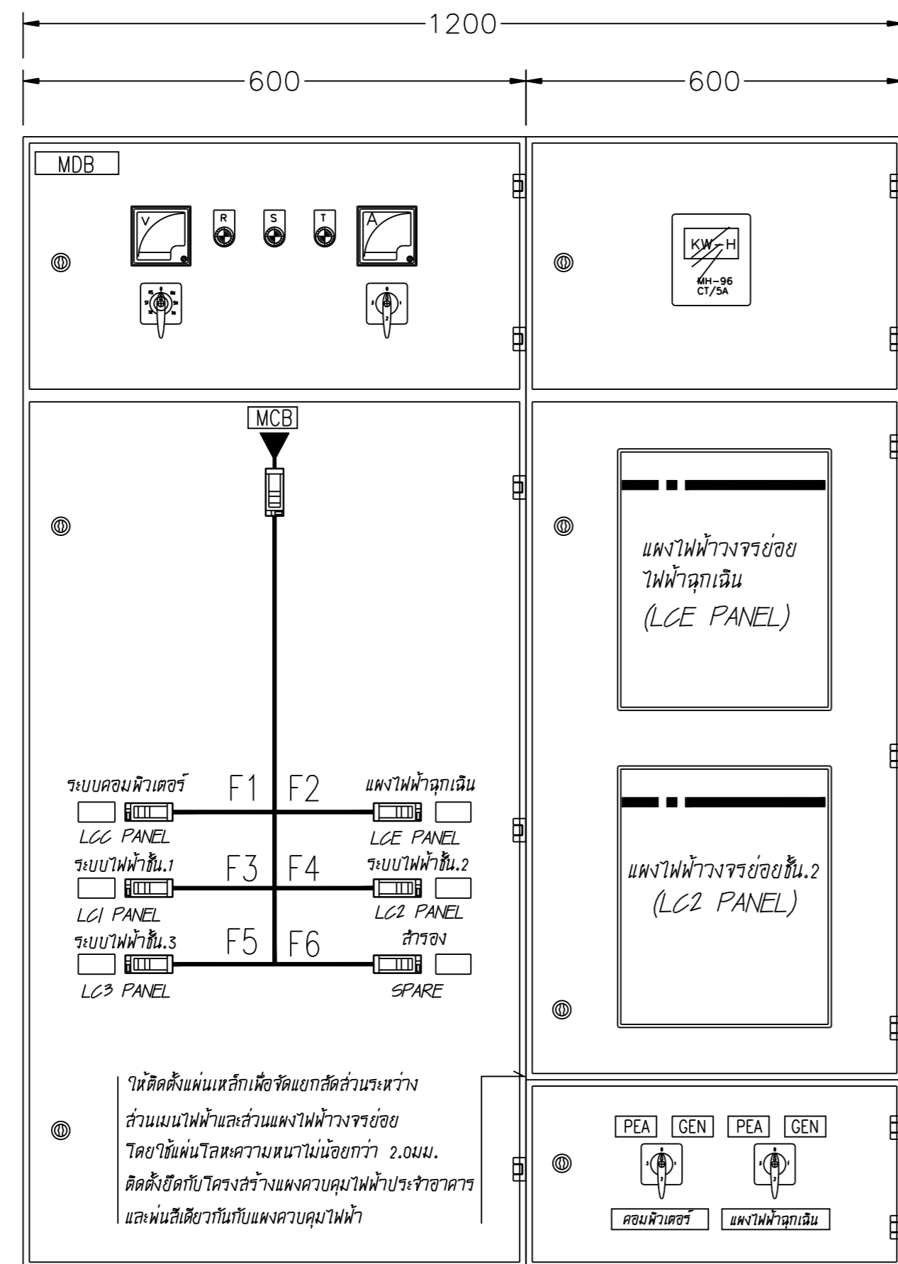
FRONT VIEW.
