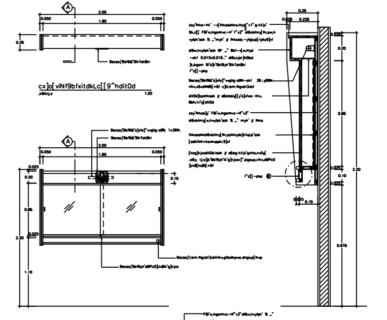
2-2 - 1/20
