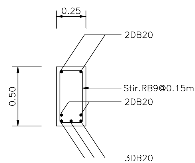
SECTION ② SCALE 1:25
