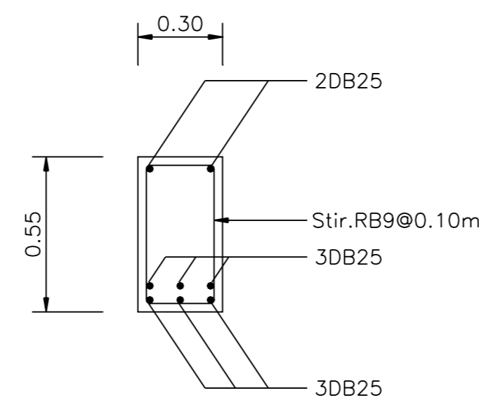
SECTION ④ SCALE 1:25
