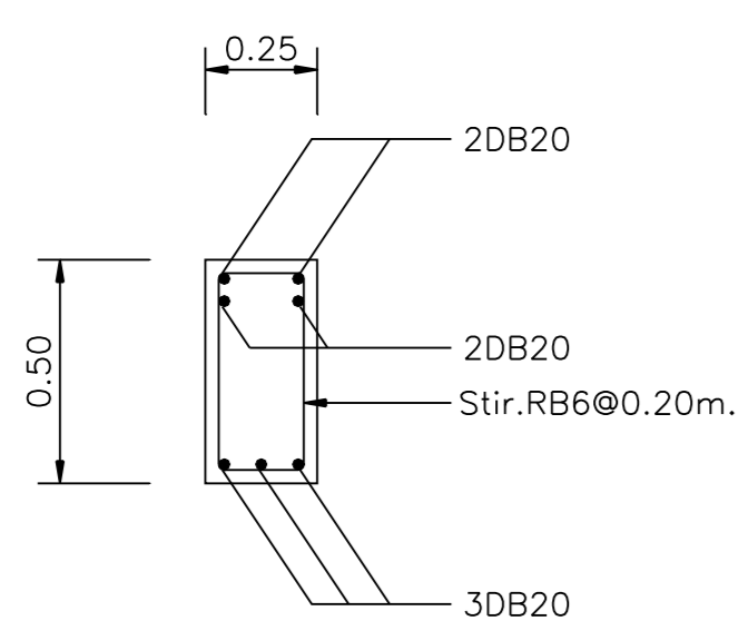
SECTION ① SCALE 1:25
