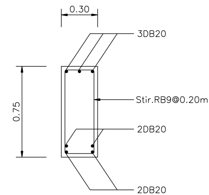
SECTION ⑤ SCALE 1:25
